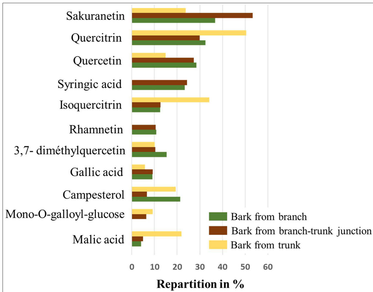
Fig. S1 - Main chemical compounds found in ethanol extracts from bark wood (AF and FC), according to the sample position in walnut trees.
