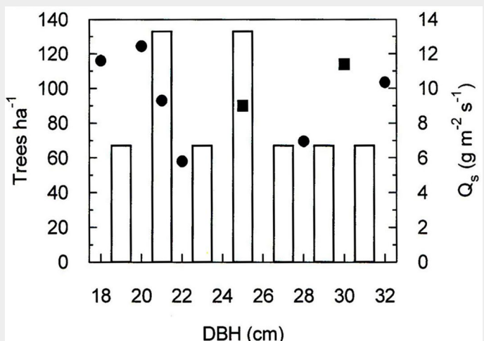
Fig. 1 - Stocking density (trees ha -1 ) at the study site (open bars) and daily maximum sap flow density ( Q_s ) of the selected study trees during the growing seasons 2007-2009 (squares) and 2011-2012 (circles) in relation to diameter at breast height (DBH).
