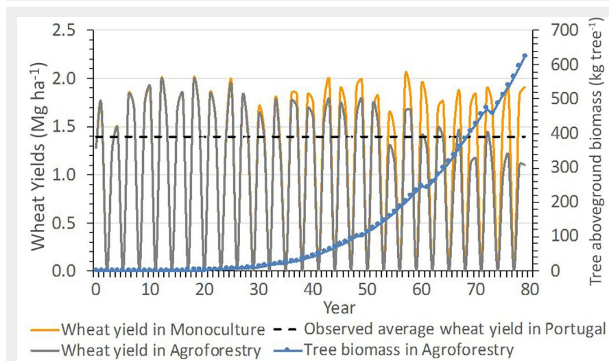
Fig. 2 - Tree growth and wheat yields simulated by the Yield-SAFE model for a wheat monoculture (wheat yield in monoculture) and an agroforestry system (wheat yield in agroforestry and tree biomass in agroforestry) combining wheat and cork oak trees in Portugal, compared to the observed average yield in Portugal for the period 1990-2011 by Almeida & Maças (2016 – observed average wheat yield in Portugal).
