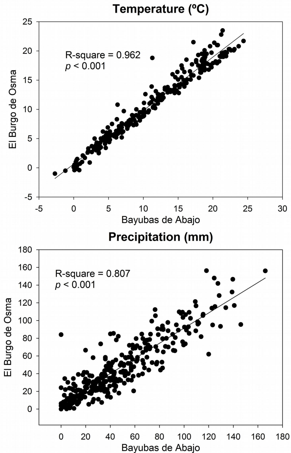
Fig. S1 - Linear regressions that relate temperature and precipitation data from El Burgo de Osma and Bayubas de Abajo weather stations.
