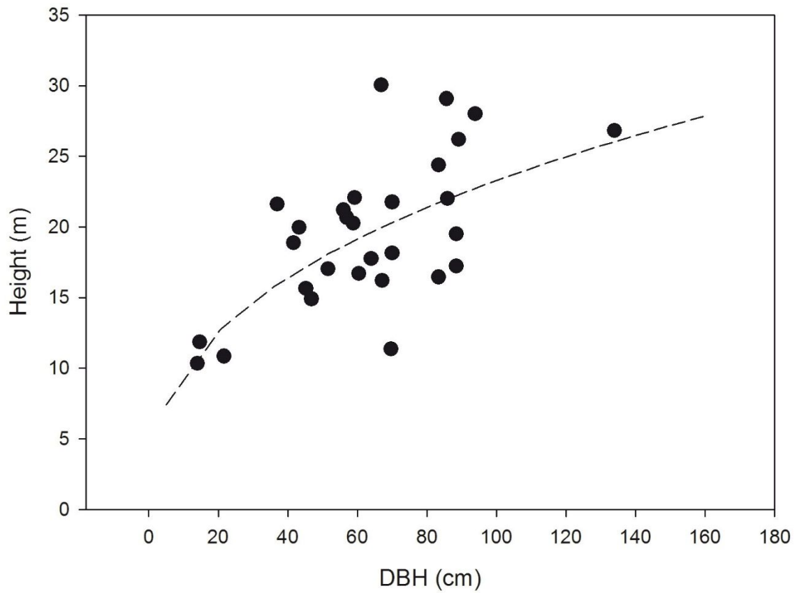
Fig. S1 - Correlation between LiDAR maximum plot heights (m) and maximum diameter measured at field plots in Poás National Park (Costa Rica).
