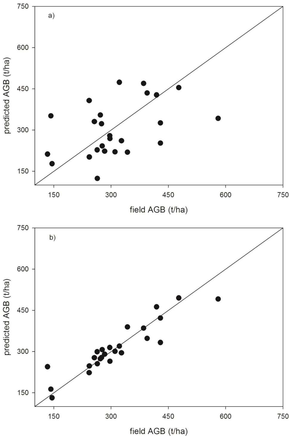
Fig. S2 - Fitting local Poás model with TCH-derived basal area (a) resulted in greater deviations than fitting with field measured basal area (b).
